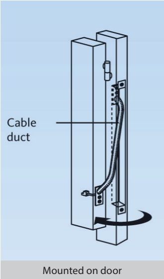
Concealed Cable Duct
