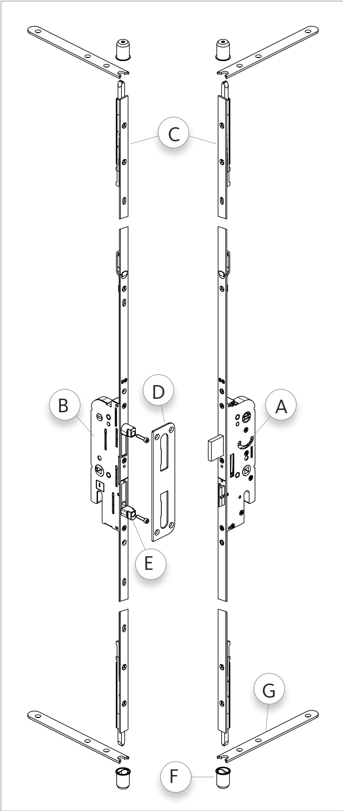
Full 1" shootbolts offer deeper penetration into the head and sill
