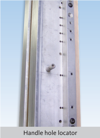
Handle hole locator
