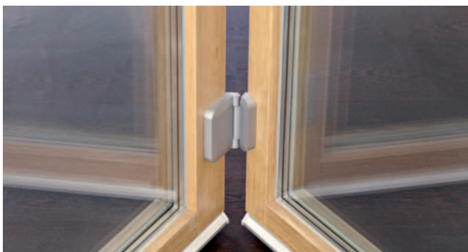
Height-adjustable sash hinge, view from outside; the screw connection is concealed from the outside which increases burglar inhibition
