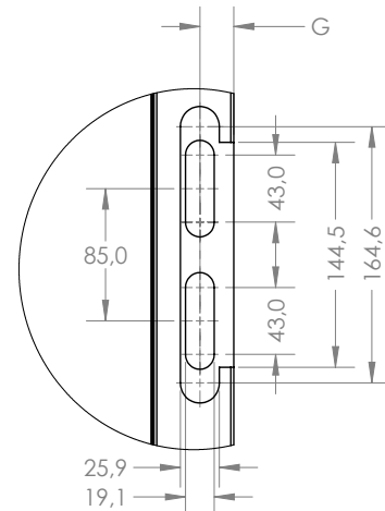
DETAIL H
